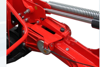
YARIM KİLİT MEKANİZMASI HALF LOCK MECHANISM
